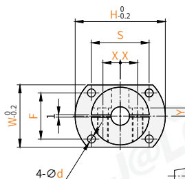
Opposite side flange type BETK-C2E1/C2N1/S1W-D
