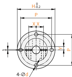
Round flange type BETK-C2E1/C2N1/S1W-Y
