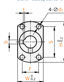
Opposite side flange type BETJ-C2E1/C2N1-D
