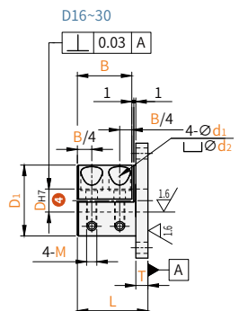
Round flange type BETK-C2E1/C2N1/S1W-Y
